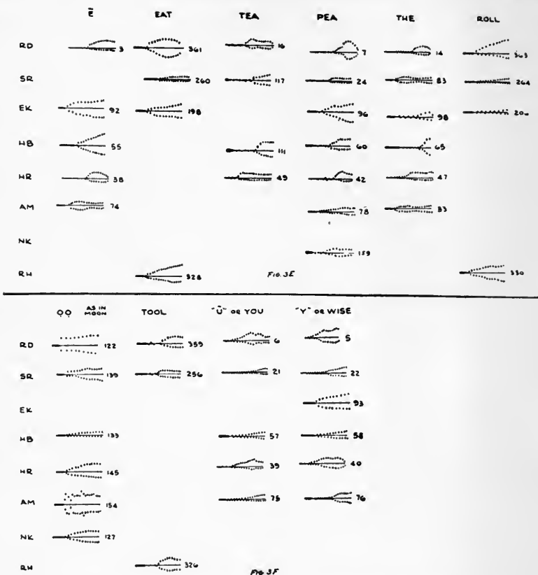
FIG. 3 (Continued). Tracings of oscillograms of speech sounds.
